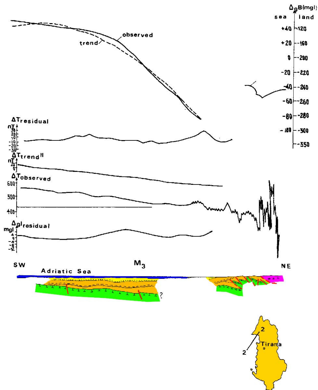
Fig. 11. Geological- geophysical profile: Adriatic Sea- Vrith
