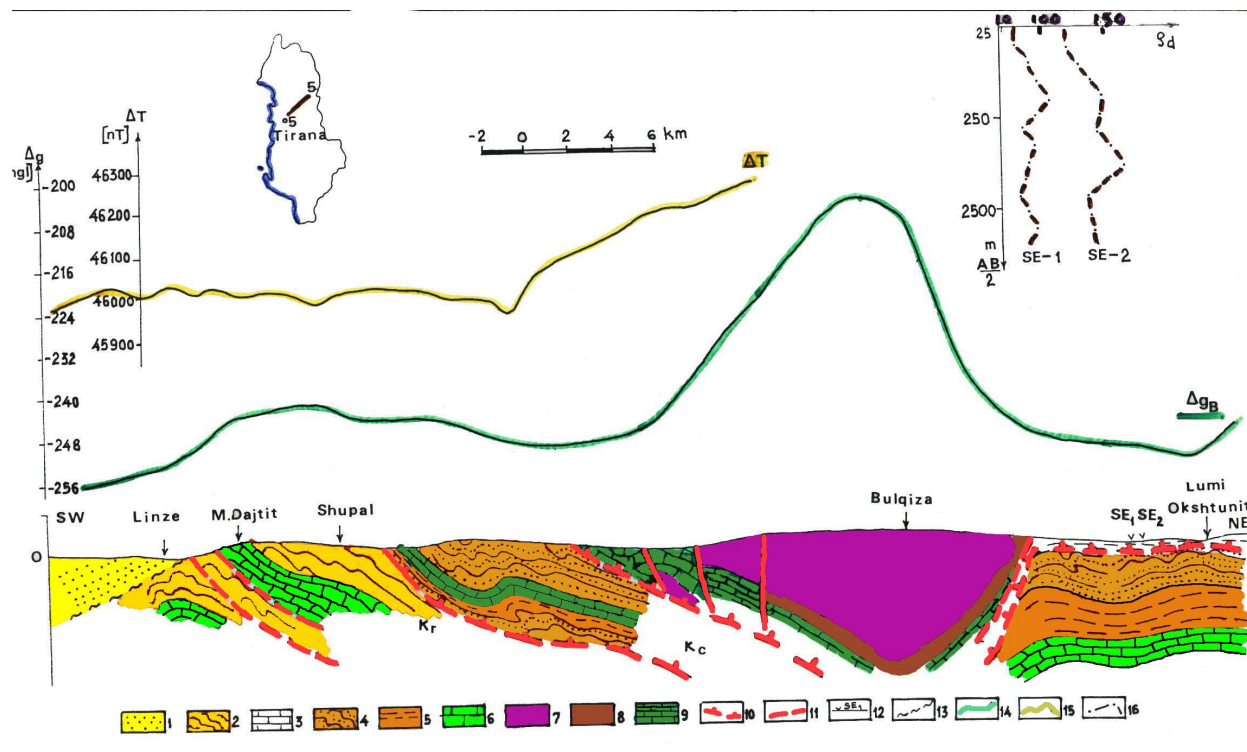
Fig. 13. Geological-geophysical profile: Tirana- Bulqizë- Shupenzë.
