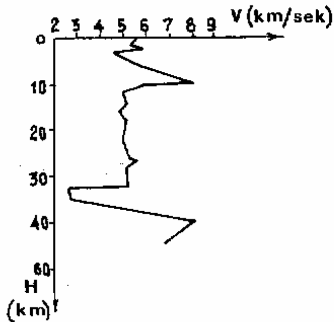
Fig. 17. Inversion of seismic P waves velocity from seismologic data (After Koçiu S., 1989).
