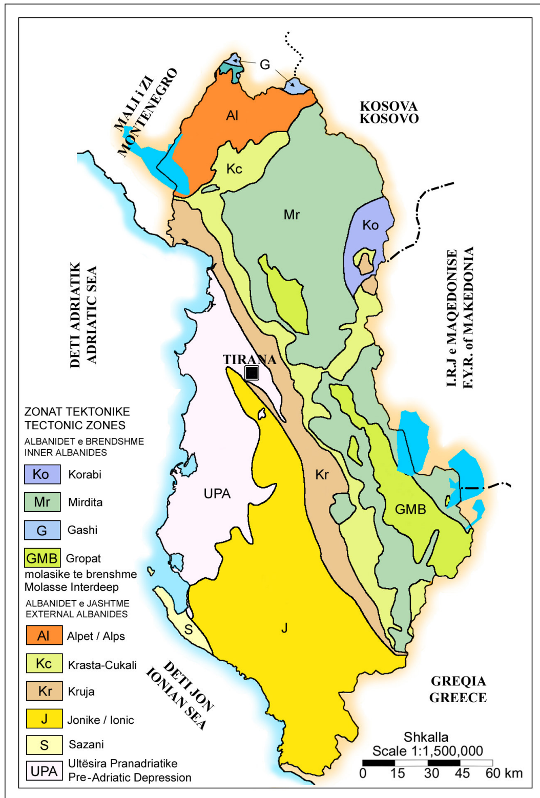
Fig. 2. Schematic Tectonic Map of Albania.
