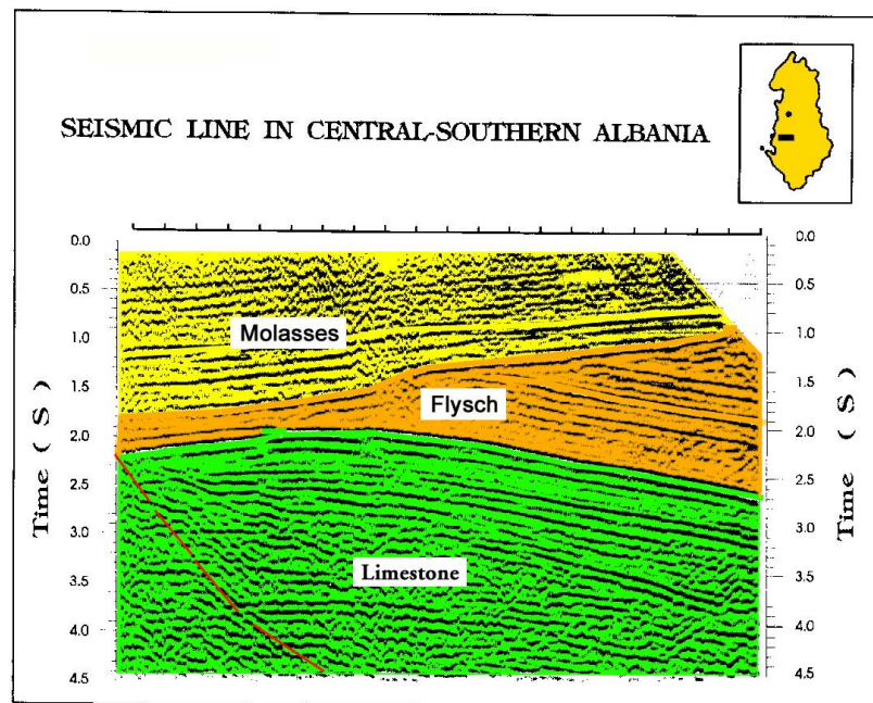
Fig. 20. Regional reflection seismic line in Ionian and Peri-Adriatic Depression.
