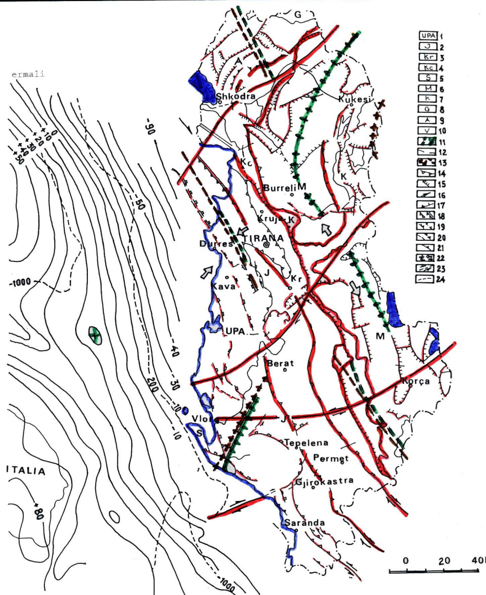
Fig. 6. The Complex Tectonic Map and axes of the Bouguer anomaly in the Albanianides and in continental plate of the Adriatic Sea.
