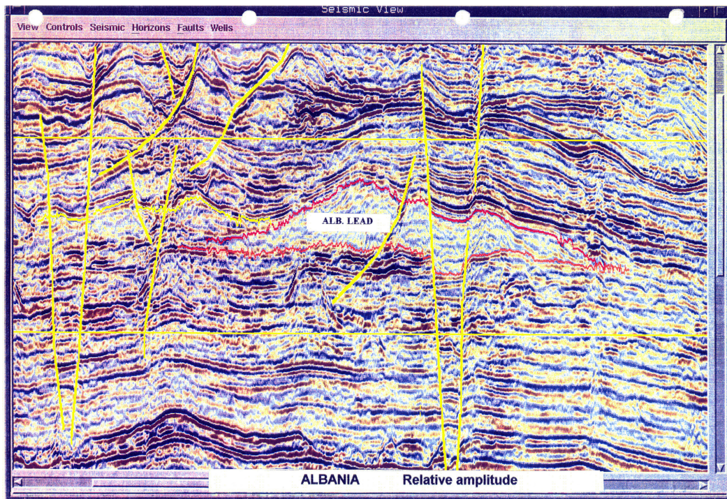
Fig. 24-b. Seismic line in Peri-Adriatic Depression (After AKH).
