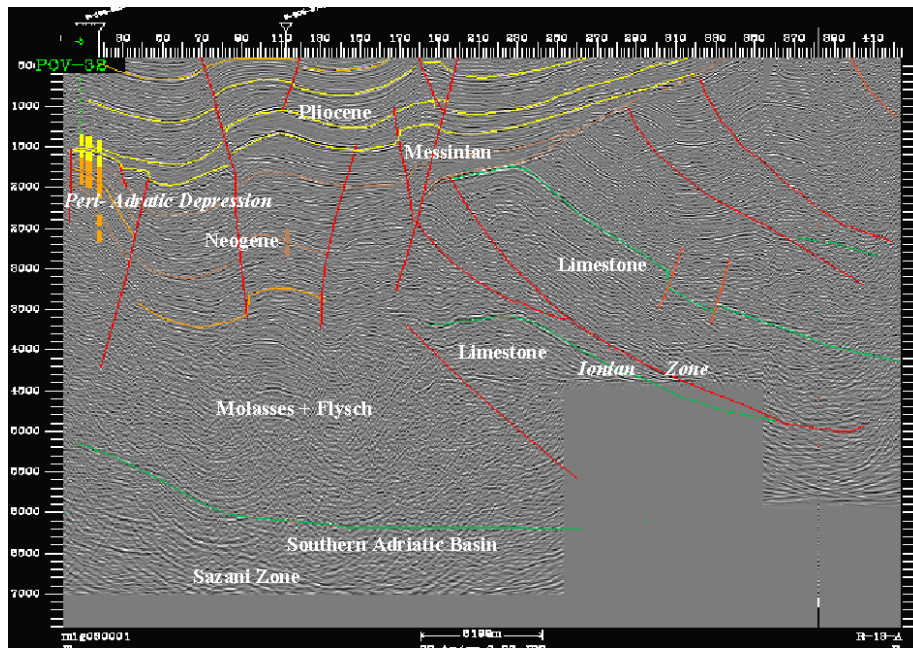
Fig. 20. Regional reflection seismic line in Ionian and Peri-Adriatic Depression.
