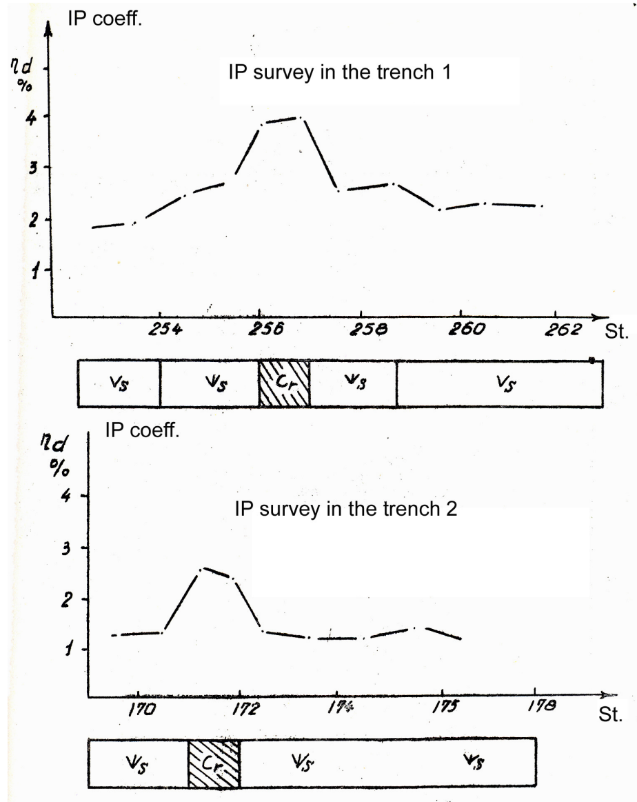
Fig. 4.20. IP anomalies according to parametric measurements over two trenches at Qafë Gjelas chrome deposit (Prenga Ll. et al. 1983). a - Complicated anomaly over the ore body and dunitic envelope, b - Single anomaly over the ore body.
