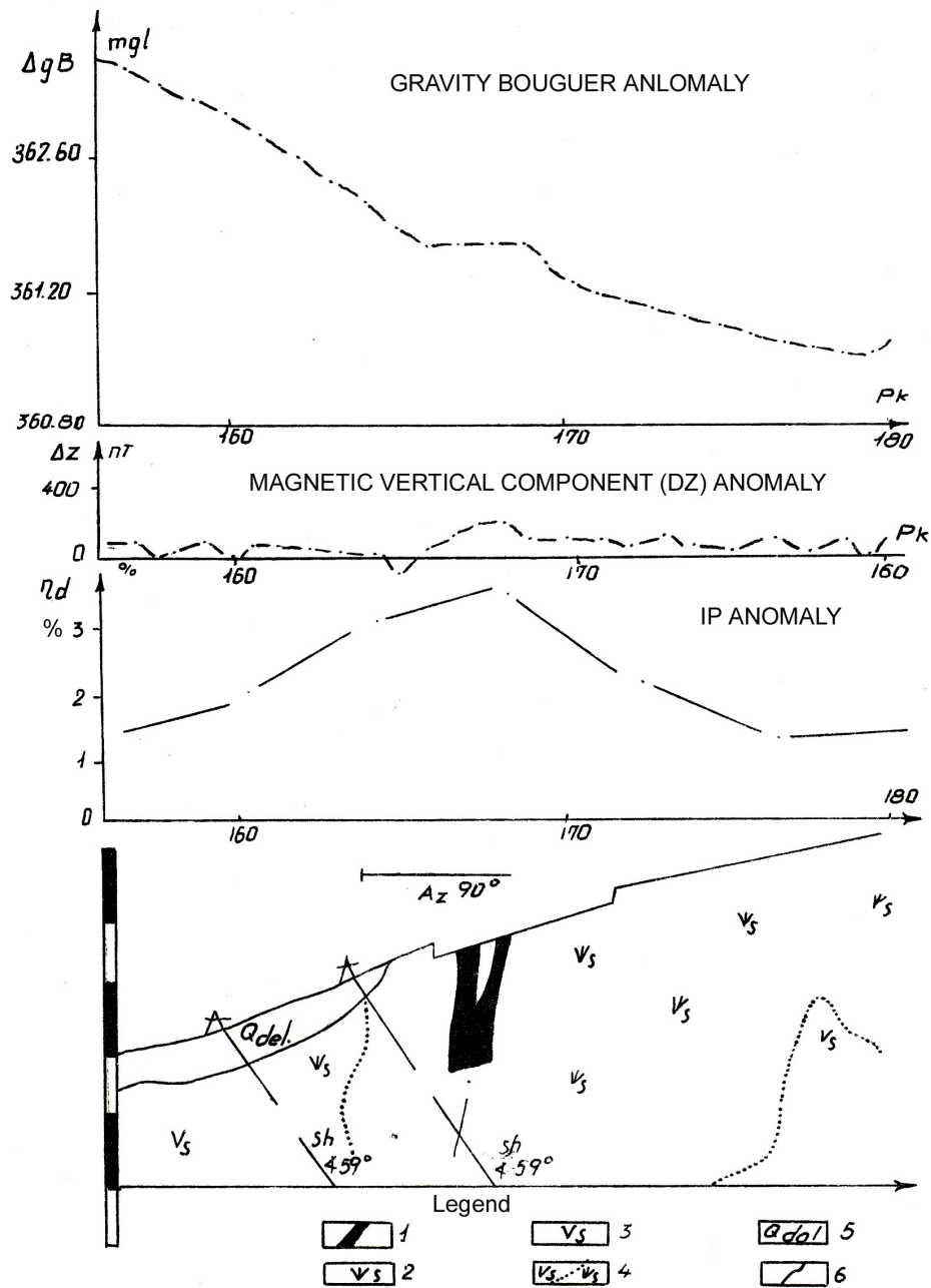
Fig. 4.19. Geological-Geophysical section in Qafe Gjela deposit (Bulqiza massif) (Prenga Ll. et al. 1983).
