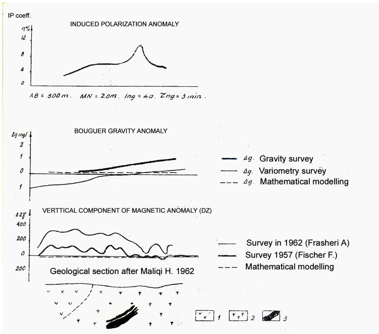
Fig. 4-4. Geological-geophysical section, Kami chromite deposit, Tropoja ultrabasic massif. (Fraseri A. et al. 1971). 1- Peridotites; 2- Dunites; 3- Chrome spinel ore body.
