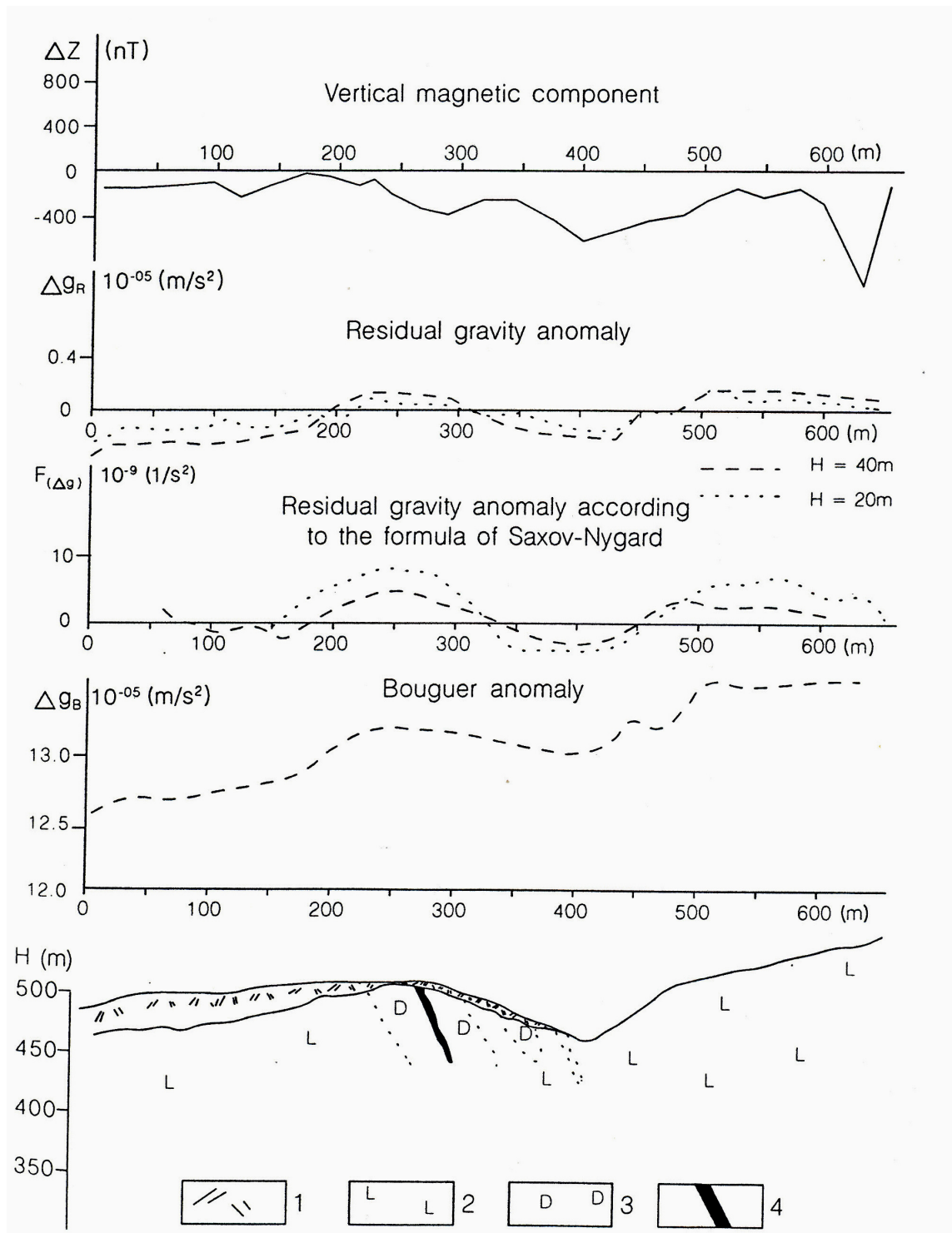
Fig. 4-7. Gravity and magnetic anomalies, Kepeneku deposit in Tropoja ultrabasic massif. (Lubonja L. and Kosho P. 1974). 1- Overburden; 2- Harzburgite; 3- Dunites; 4- Chromite ore body.
