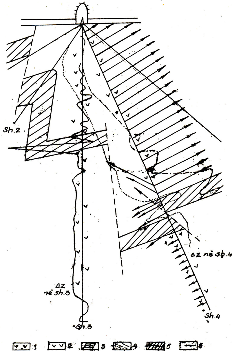
Fig. 4.27. Geomagnetic section according to three component borehole magnetic surveys in Bulqiza chrome deposit (Gjevrekü Dh. 1984). 1- Dunite; 2- Hartzbourgite; 3- Ore body; 4- Vertical magnetic component ( \Delta Z ) plot; 5- Total vector of the magnetic field intensity ( \Delta T ).
