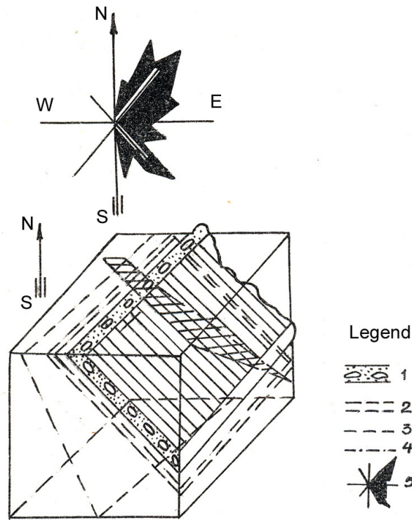
Fig. 4.32. Primary structural elements and the direction of the axis of magnetic micro anomalies. (Frasheri et al. 1969). 1 - Banded texture; 2 - Primary fissure system L, 3 - Primary fissure system S, 4 - Primary fissure system Q, 5 - Rose diagram and vectors of the direction of the magnetic micro anomalies axis.
