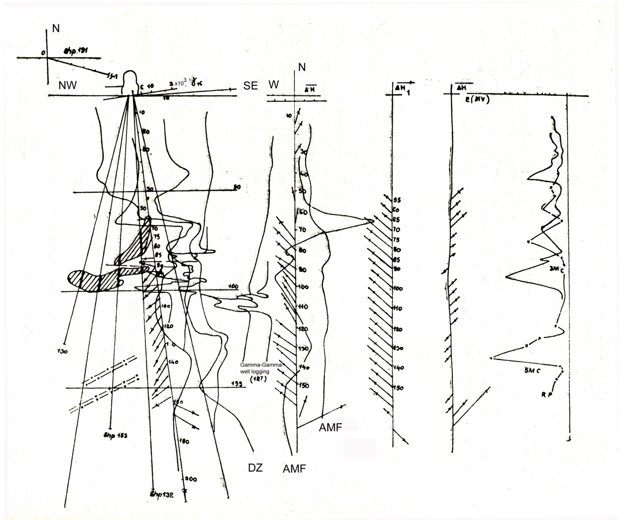
Fig. 4.26. Geological-geophysical section in L-L 5 underground magnetic survey line, Shkalla deposits, Bulqiza ultrabasic massif. (Langora Ll. Et al. 1989)
