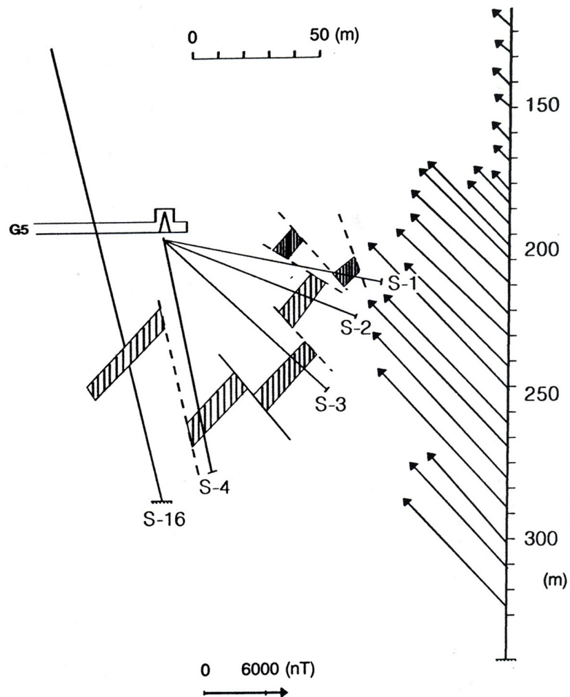
Fig. 4-28. Anomaly of total magnetic field intensity ( \Delta T ), according to the three-components borehole magnetic field surveys for underground exploration of chromite ore (Gjevreku Dh., 1984, Lubonja L. et al. 1995).
