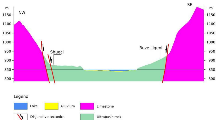
Fig. 6. Geological Profile through Micro Prespa Lake
