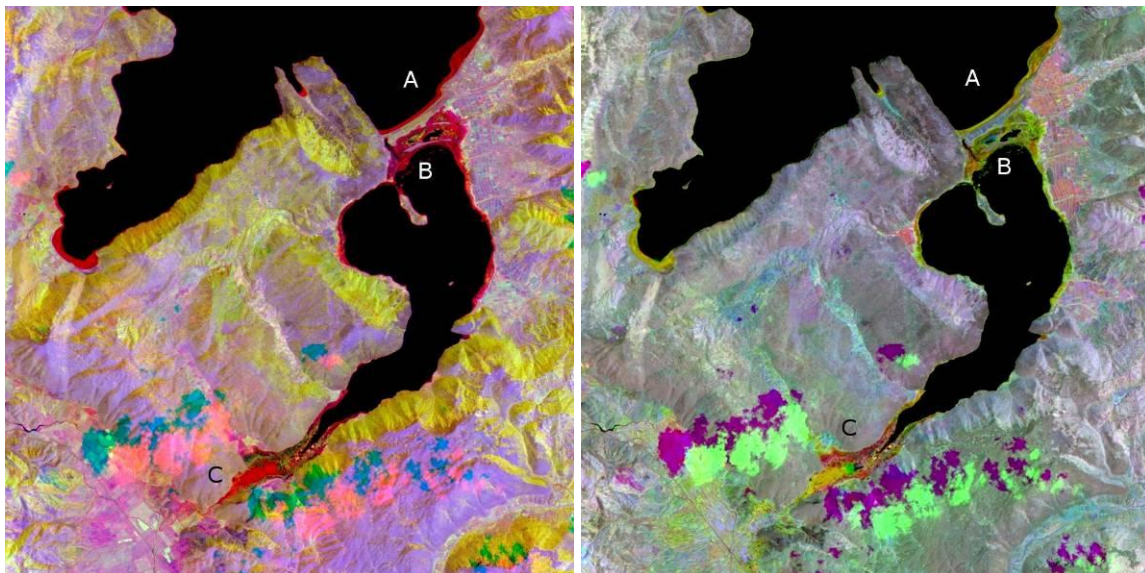
Fig Ccc – Combination of NIRS bands (left: 1973-1987-2002, right 1987-2002-2010)
