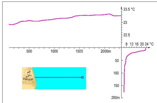
Fig. 4. Water temperature of Ohrid lake.
