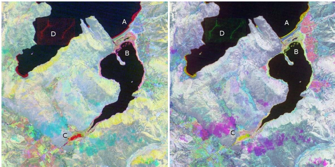
Fig Ddd – Combination of NDVI (left: 1973-1987-2002, right 1987-2002-2010)
